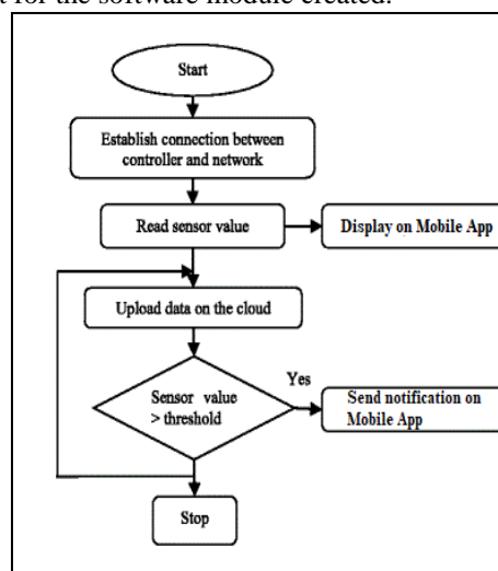
Figure 7: Flowchart for software development
